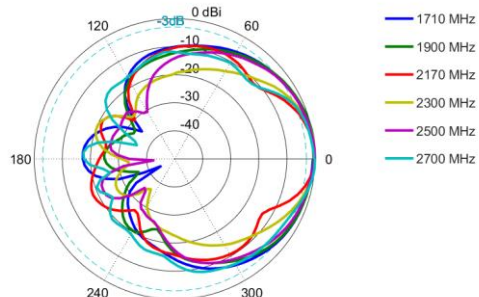
Elevation: 1710 – 2700 MHz
